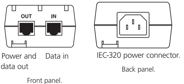
Figure 2. Ports on the power injector.
